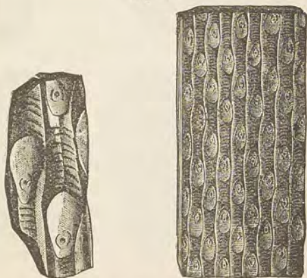
SIGILLARIA GREESERI (Coal Measures.)
